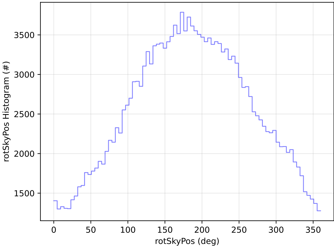
ddf_acor_sf10_lsf20_lsr10_v3.4_10yrs All sky g band: rotSkyPos Histogram
