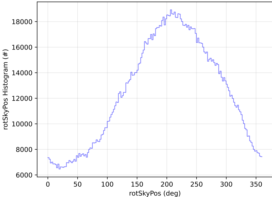
ddf_acor_sf10_lsf20_lsr10_v3.4_10yrs All sky all bands: rotSkyPos Histogram
