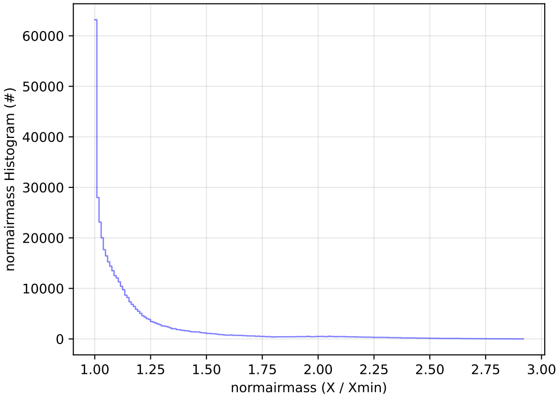
ddf_acor_sf10_lsf20_lsr10_v3.4_10yrs WFD z band: normairmass Histogram
