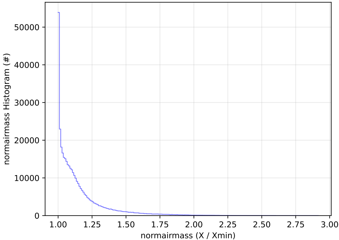
ddf_acor_sf10_lsf20_lsr10_v3.4_10yrs WFD y band: normairmass Histogram
