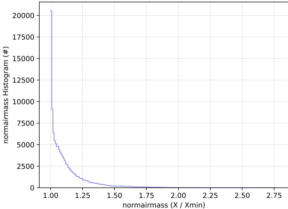
ddf_acor_sf10_lsf20_lsr10_v3.4_10yrs WFD u band: normairmass Histogram
