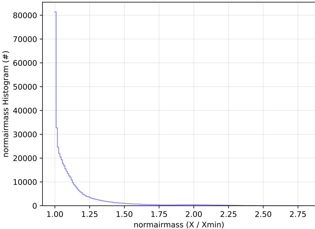
ddf_acor_sf10_lsf20_lsr10_v3.4_10yrs WFD r band: normairmass Histogram
