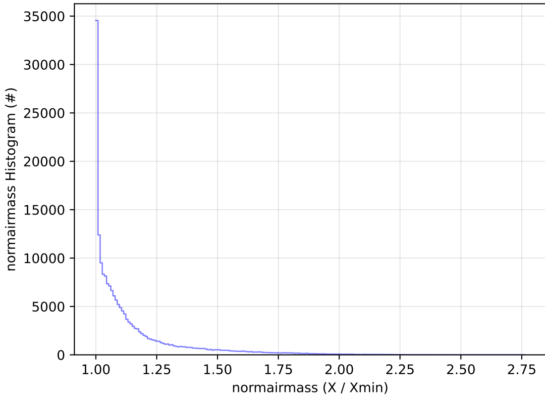
ddf_acor_sf10_lsf20_lsr10_v3.4_10yrs WFD g band: normairmass Histogram
