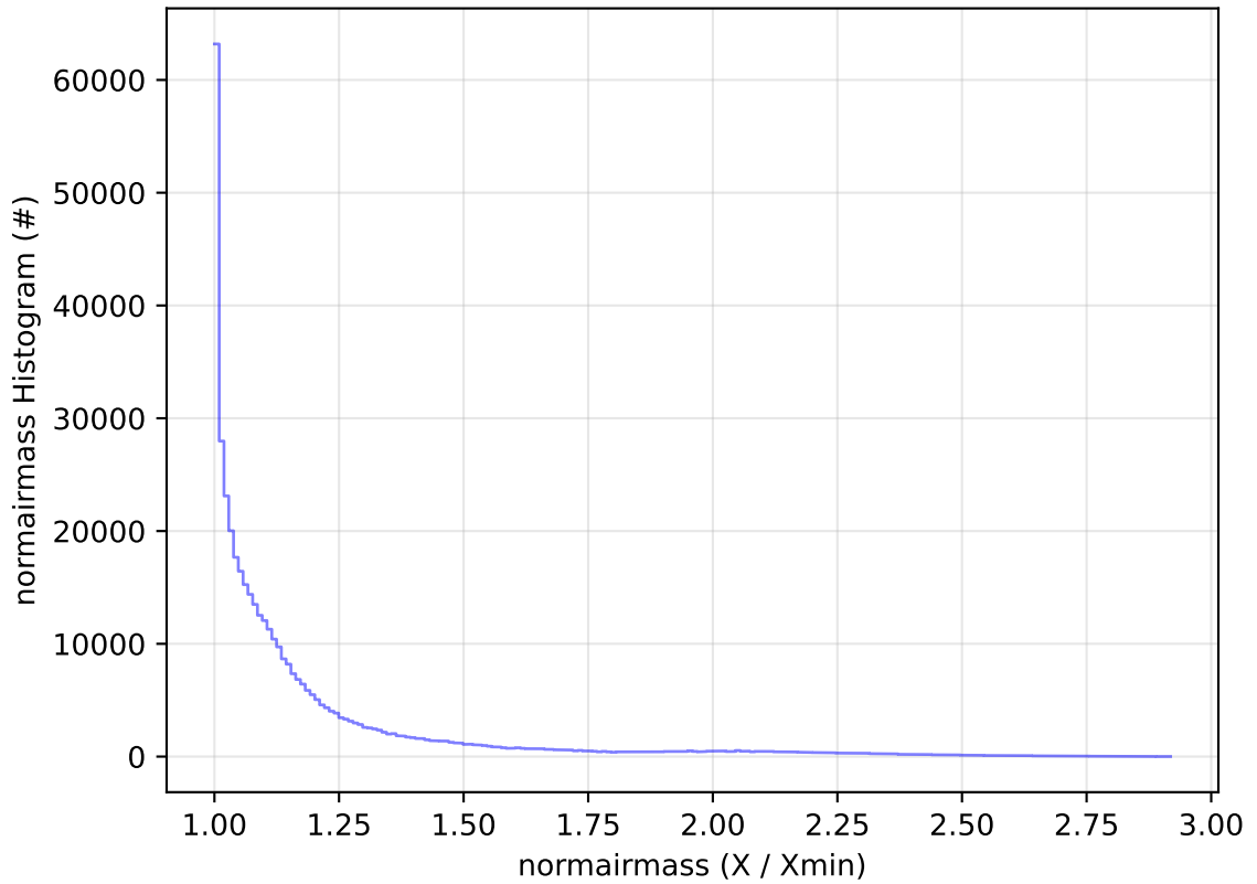
ddf_acor_sf10_lsf20_lsr10_v3.4_10yrs All sky z band: normairmass Histogram
