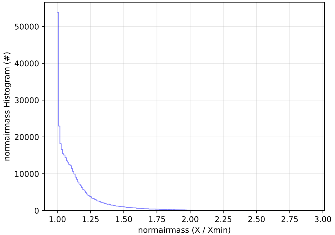
ddf_acor_sf10_lsf20_lsr10_v3.4_10yrs All sky y band: normairmass Histogram
