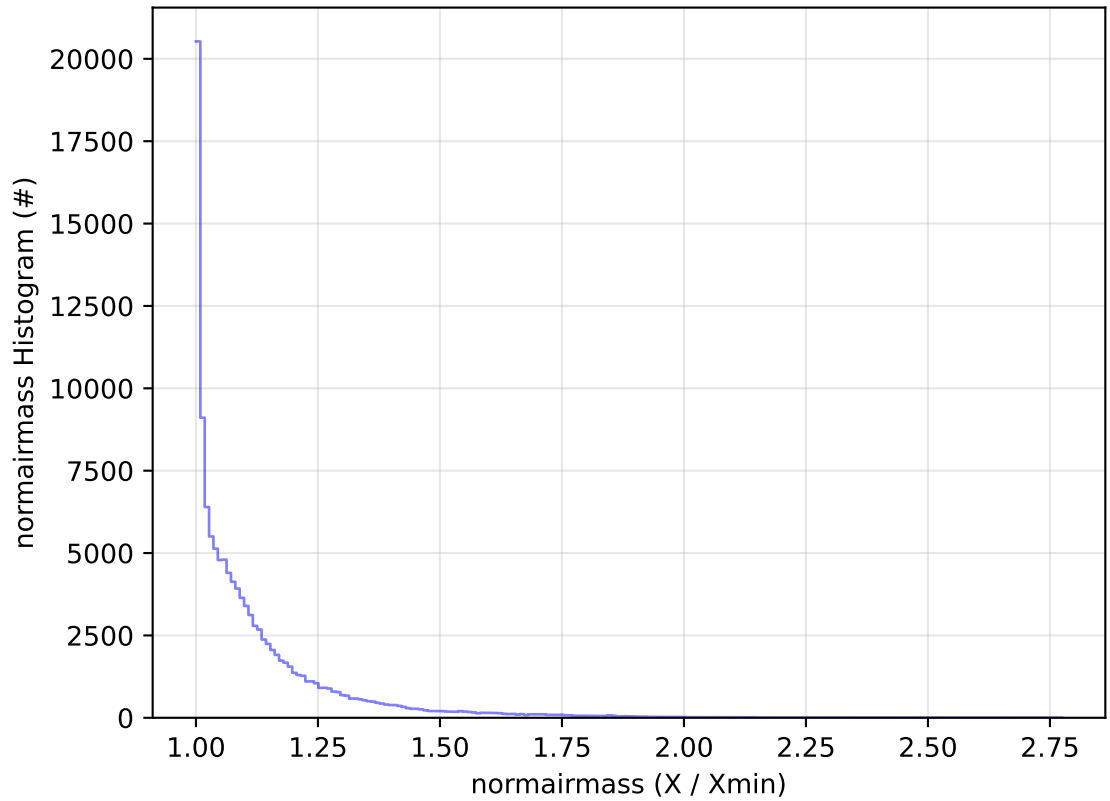
ddf_acor_sf10_lsf20_lsr10_v3.4_10yrs All sky u band: normairmass Histogram
