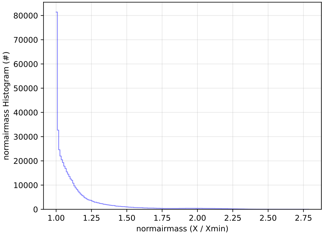
ddf_acor_sf10_lsf20_lsr10_v3.4_10yrs All sky r band: normairmass Histogram
