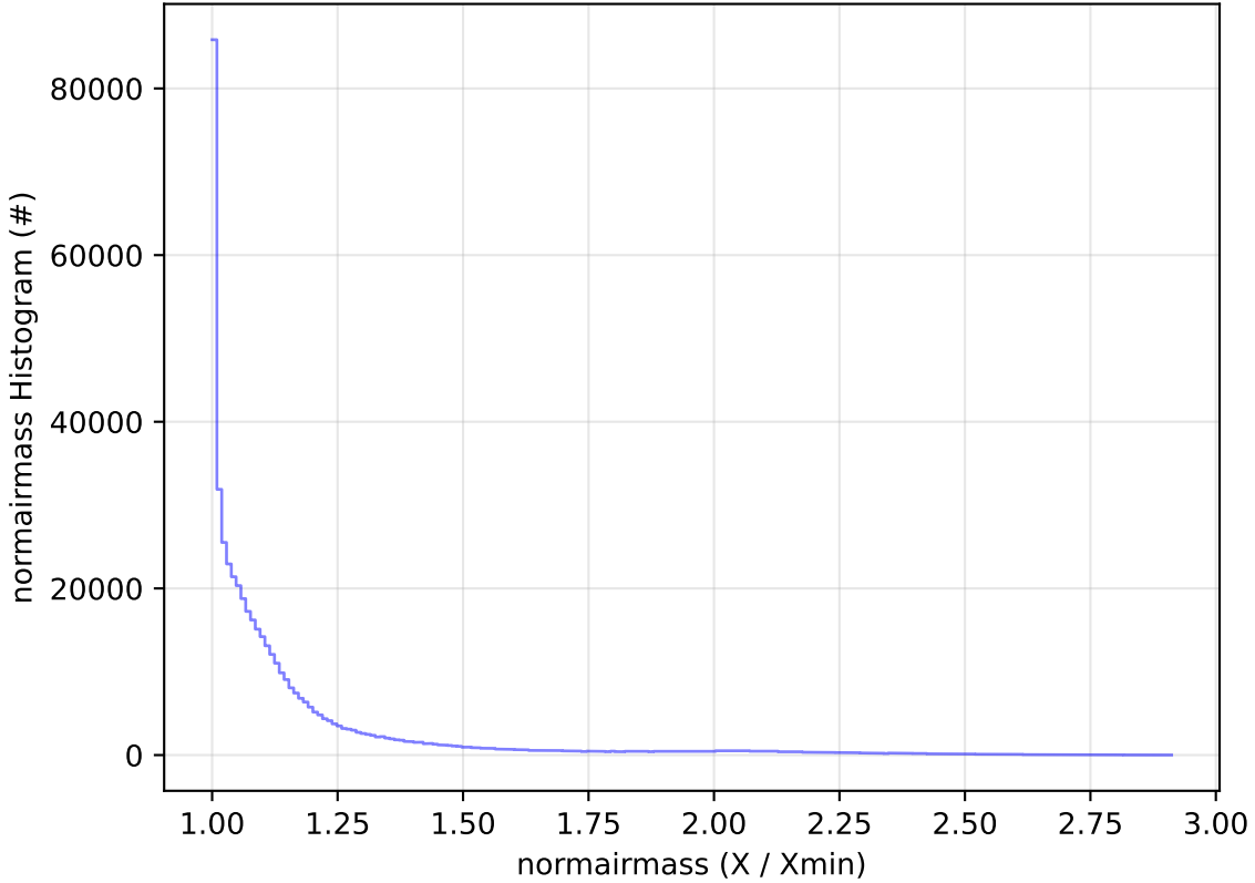
ddf_acor_sf10_lsf20_lsr10_v3.4_10yrs All sky i band: normairmass Histogram
