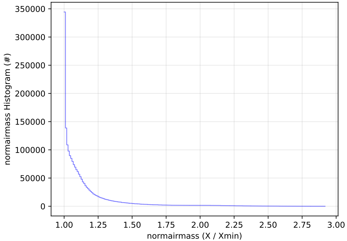
ddf_acor_sf10_lsf20_lsr10_v3.4_10yrs All sky all bands: normairmass Histogram
