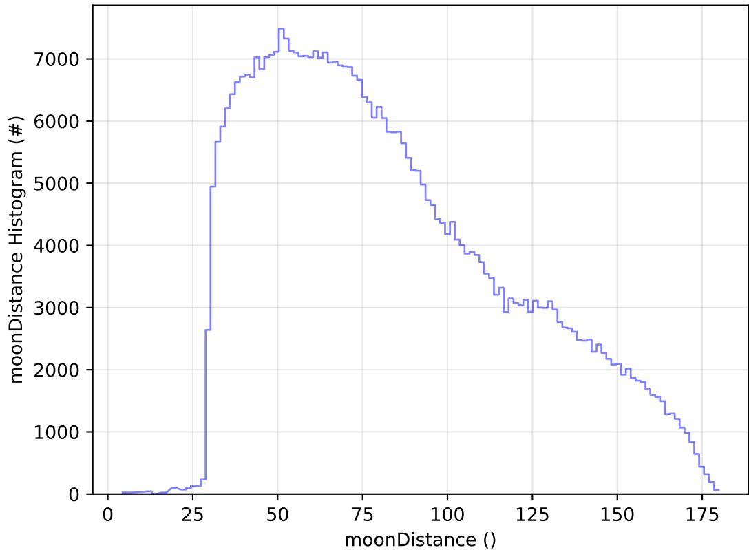
ddf_acor_sf10_lsf20_lsr10_v3.4_10yrs WFD z band: moonDistance Histogram
