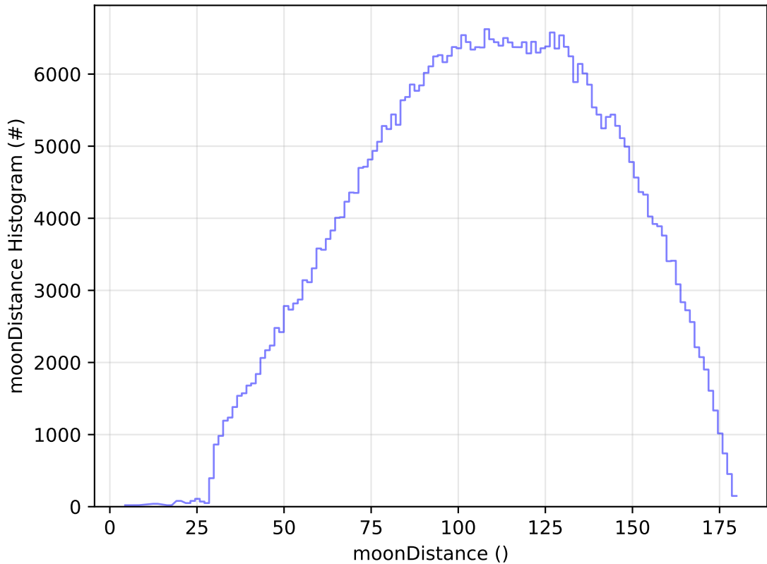
ddf_acor_sf10_lsf20_lsr10_v3.4_10yrs WFD r band: moonDistance Histogram
