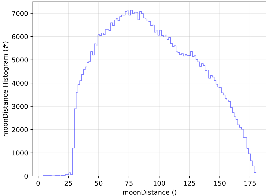
ddf_acor_sf10_lsf20_lsr10_v3.4_10yrs WFD i band: moonDistance Histogram
