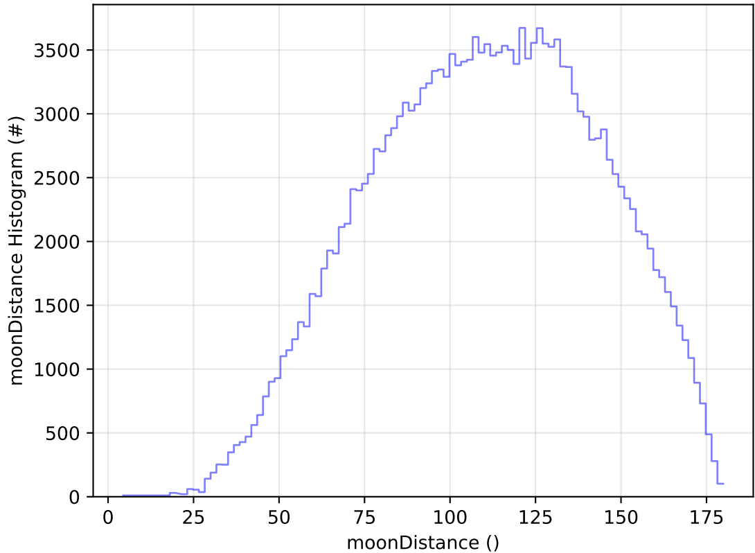
ddf_acor_sf10_lsf20_lsr10_v3.4_10yrs WFD g band: moonDistance Histogram
