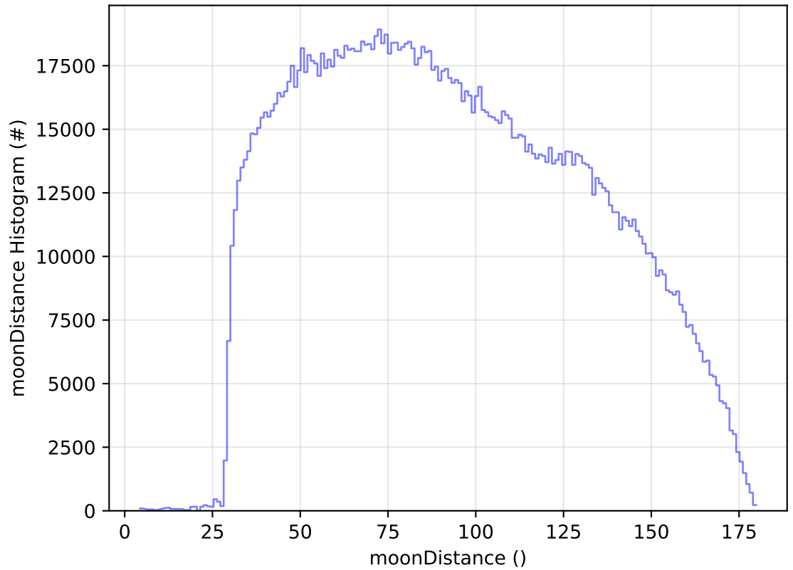
ddf_acor_sf10_lsf20_lsr10_v3.4_10yrs WFD all bands: moonDistance Histogram
