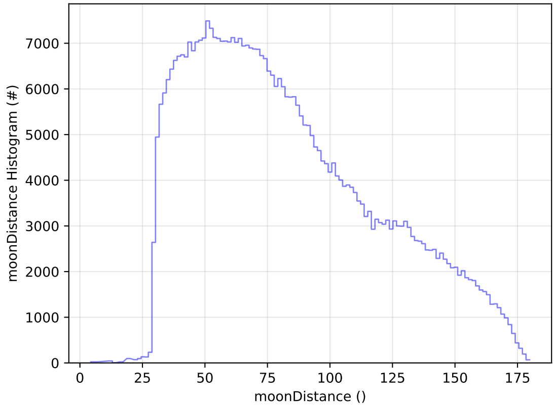
ddf_acor_sf10_lsf20_lsr10_v3.4_10yrs All sky z band: moonDistance Histogram
