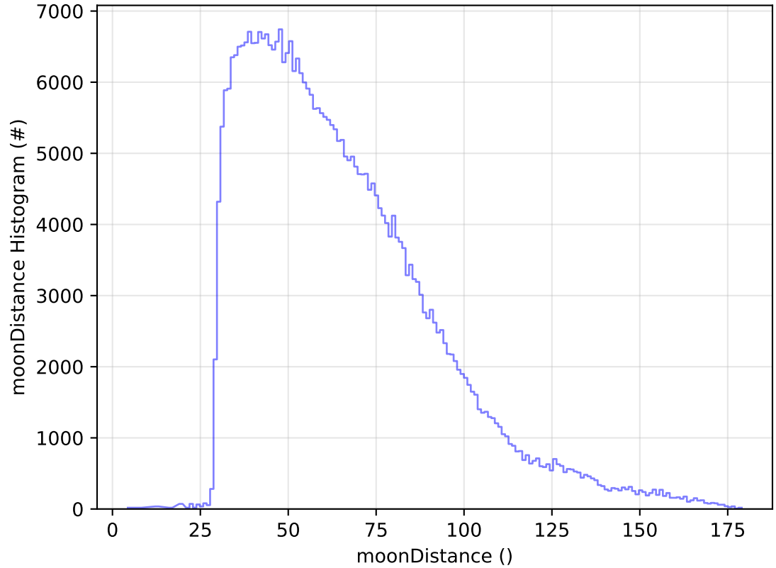
ddf_acor_sf10_lsf20_lsr10_v3.4_10yrs All sky y band: moonDistance Histogram
