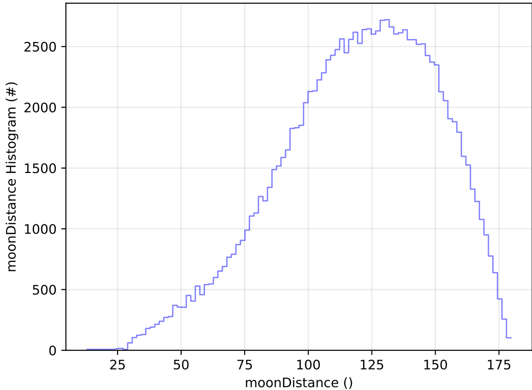
ddf_acor_sf10_lsf20_lsr10_v3.4_10yrs All sky u band: moonDistance Histogram
