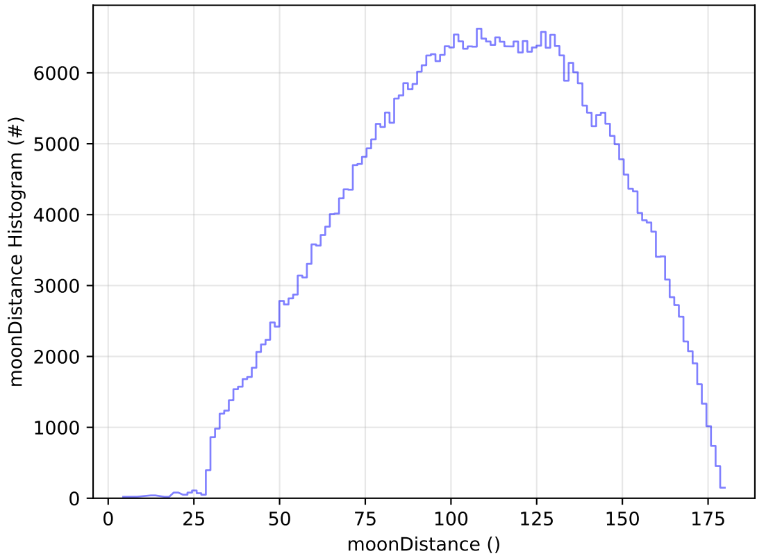
ddf_acor_sf10_lsf20_lsr10_v3.4_10yrs All sky r band: moonDistance Histogram
