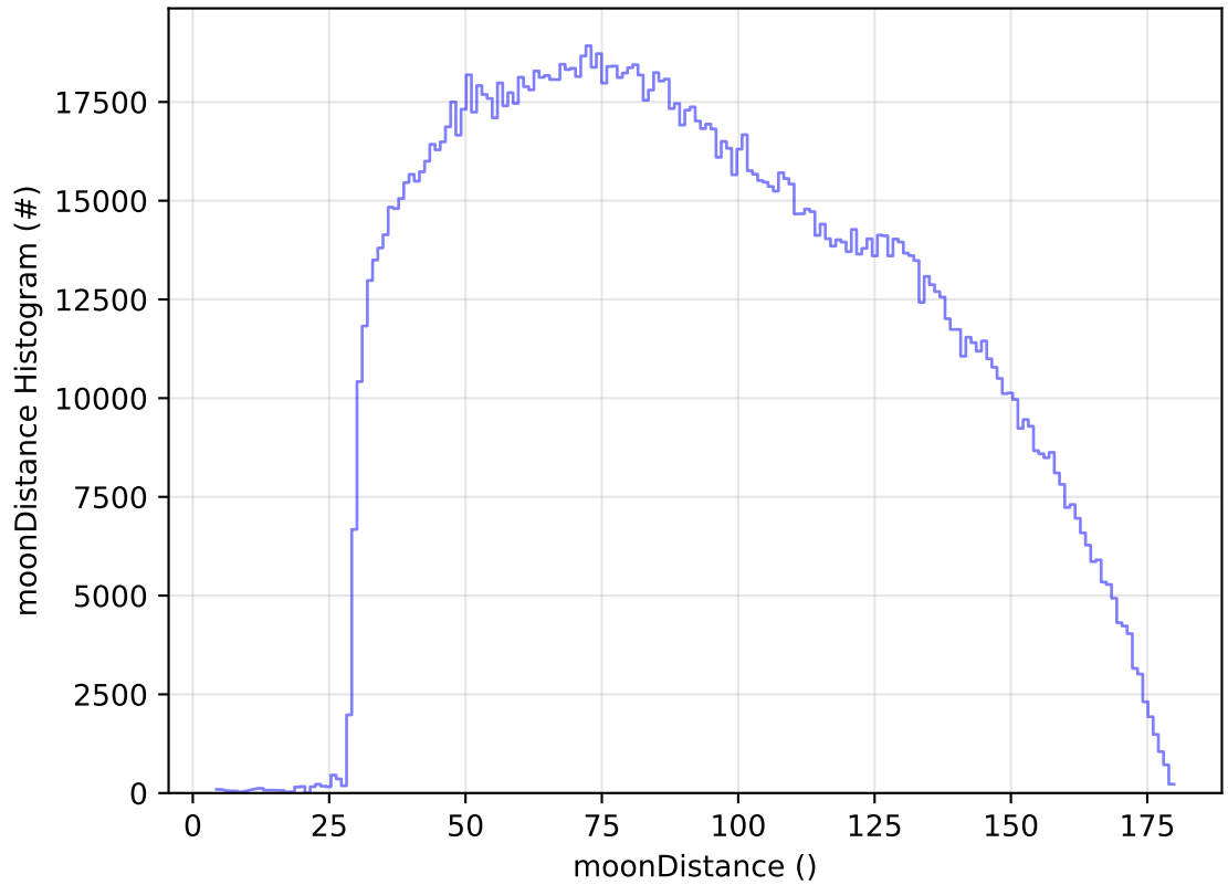
ddf_acor_sf10_lsf20_lsr10_v3.4_10yrs All sky all bands: moonDistance Histogram
