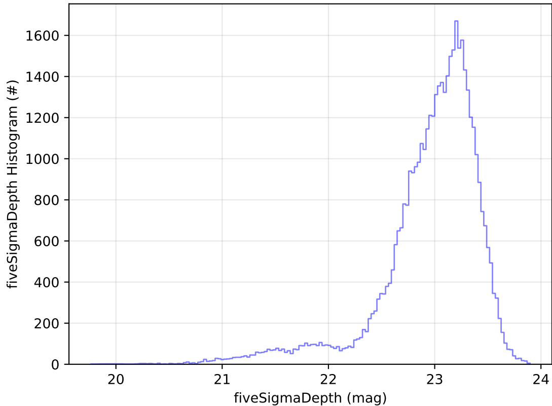
ddf_acor_sf10_lsf20_lsr10_v3.4_10yrs Yr 1 z band: fiveSigmaDepth Histogram
