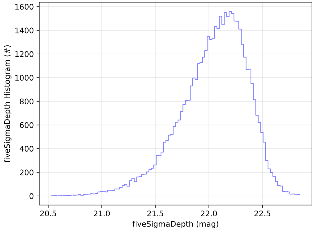
ddf_acor_sf10_lsf20_lsr10_v3.4_10yrs Yr 1 y band: fiveSigmaDepth Histogram
