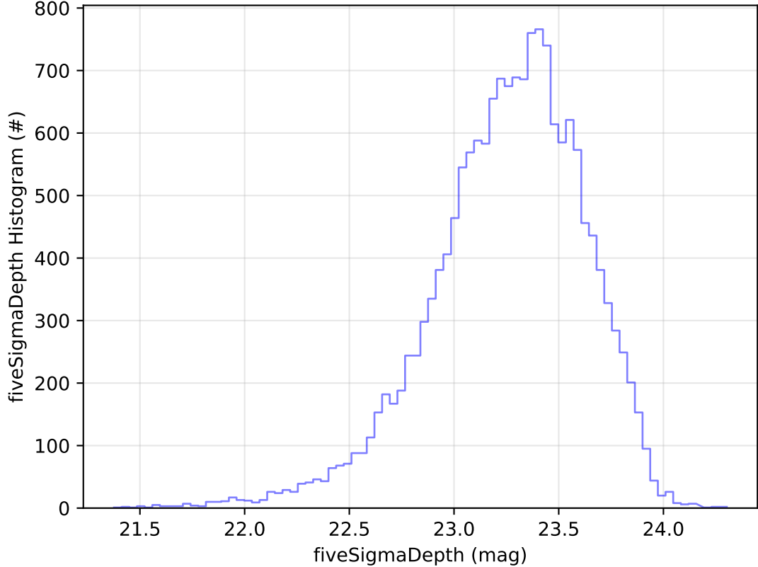
ddf_acor_sf10_lsf20_lsr10_v3.4_10yrs Yr 1 u band: fiveSigmaDepth Histogram
