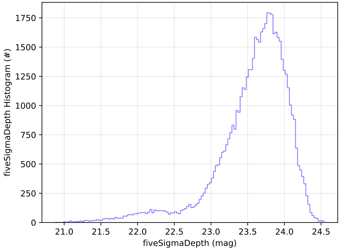
ddf_acor_sf10_lsf20_lsr10_v3.4_10yrs Yr 1 i band: fiveSigmaDepth Histogram
