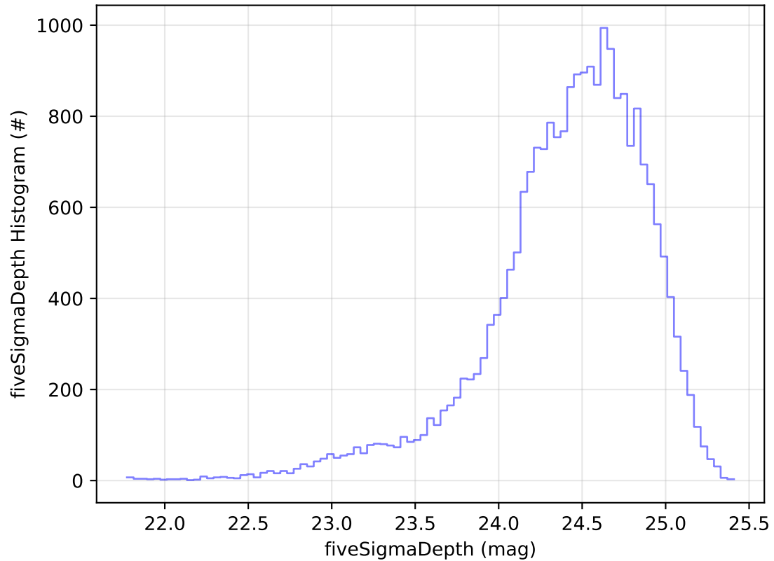
ddf_acor_sf10_lsf20_lsr10_v3.4_10yrs Yr 1 g band: fiveSigmaDepth Histogram
