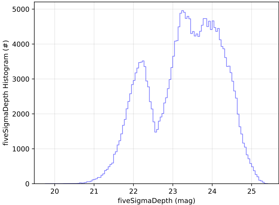
ddf_acor_sf10_lsf20_lsr10_v3.4_10yrs Yr 1 all bands: fiveSigmaDepth Histogram
