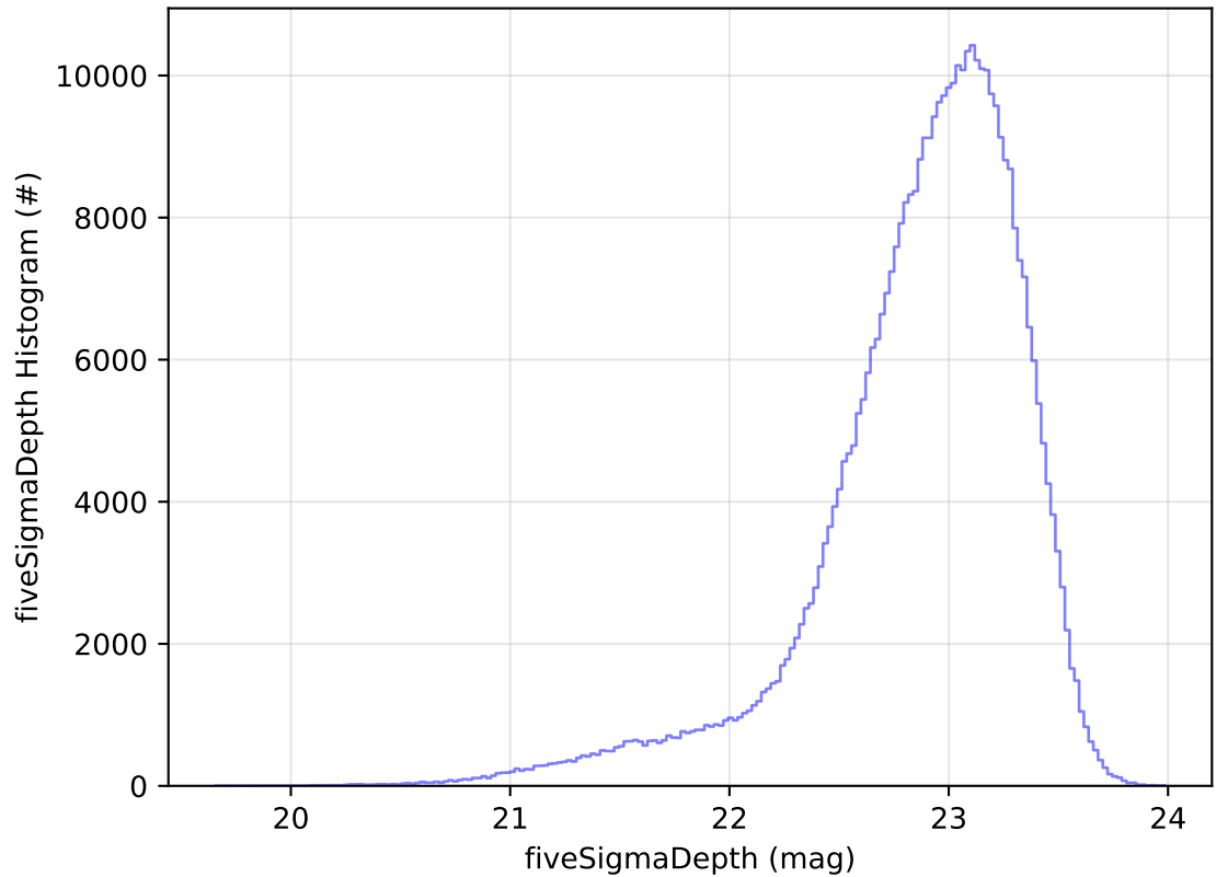
ddf_acor_sf10_lsf20_lsr10_v3.4_10yrs WFD z band: fiveSigmaDepth Histogram
