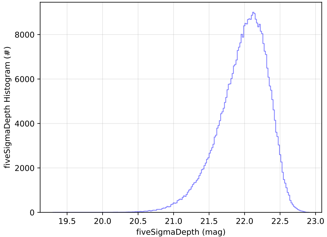
ddf_acor_sf10_lsf20_lsr10_v3.4_10yrs WFD y band: fiveSigmaDepth Histogram
