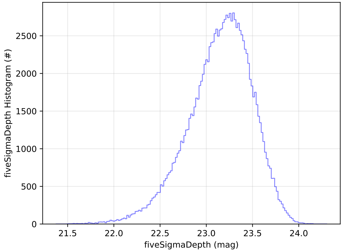
ddf_acor_sf10_lsf20_lsr10_v3.4_10yrs WFD u band: fiveSigmaDepth Histogram
