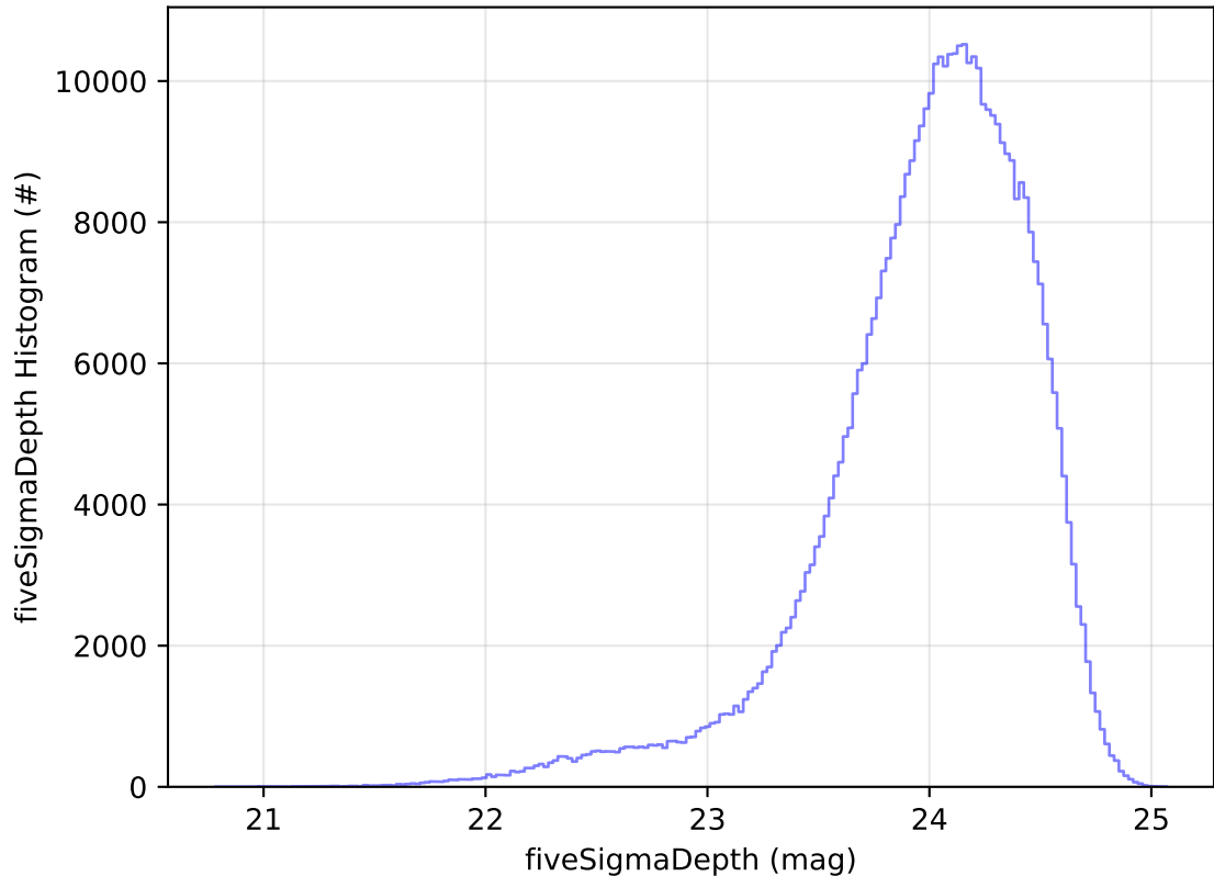
ddf_acor_sf10_lsf20_lsr10_v3.4_10yrs WFD r band: fiveSigmaDepth Histogram
