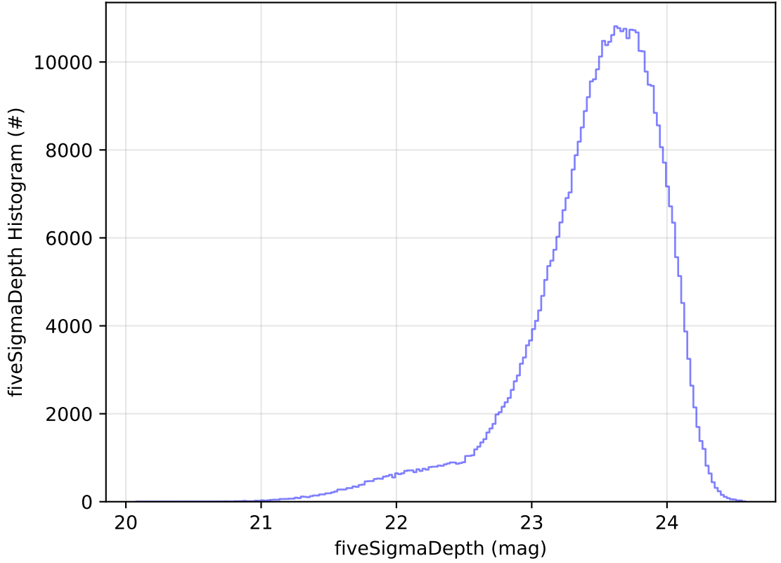
ddf_acor_sf10_lsf20_lsr10_v3.4_10yrs WFD i band: fiveSigmaDepth Histogram
