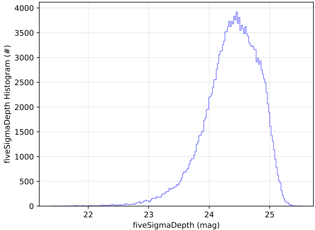
ddf_acor_sf10_lsf20_lsr10_v3.4_10yrs WFD g band: fiveSigmaDepth Histogram
