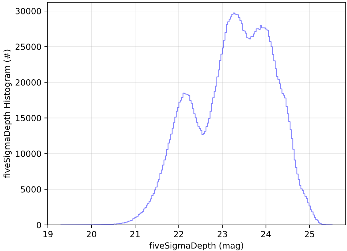
ddf_acor_sf10_lsf20_lsr10_v3.4_10yrs WFD all bands: fiveSigmaDepth Histogram
