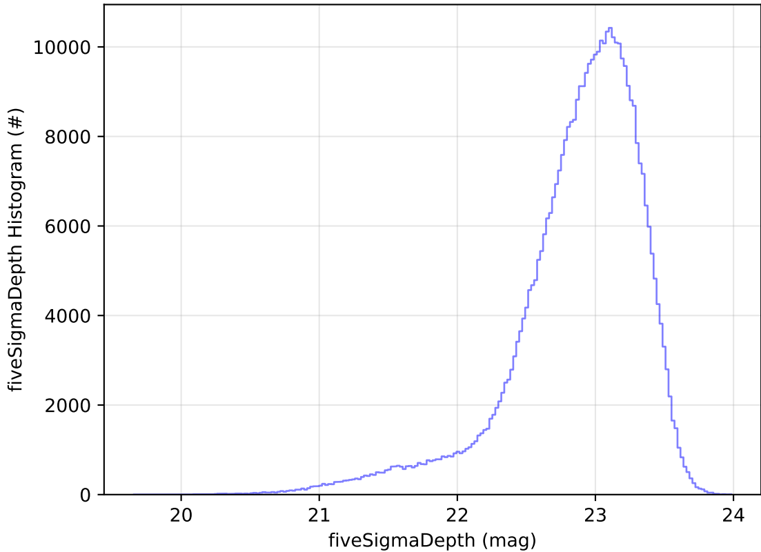
ddf_acor_sf10_lsf20_lsr10_v3.4_10yrs All sky z band: fiveSigmaDepth Histogram
