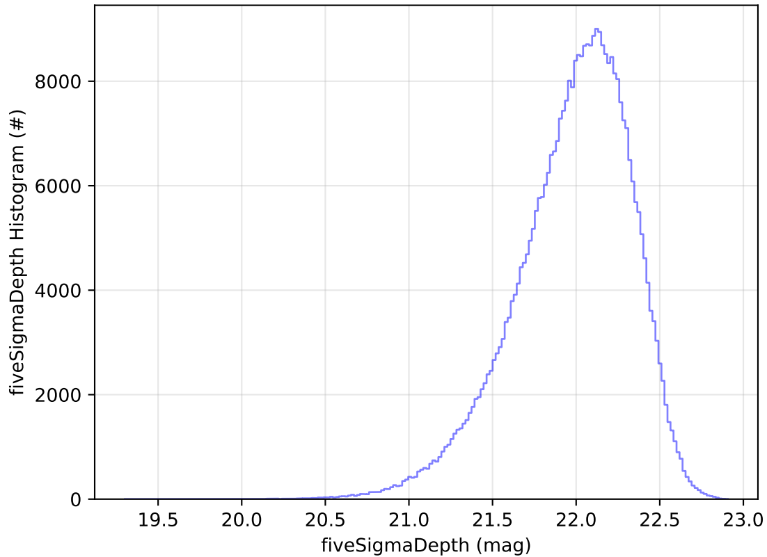
ddf_acor_sf10_lsf20_lsr10_v3.4_10yrs All sky y band: fiveSigmaDepth Histogram
