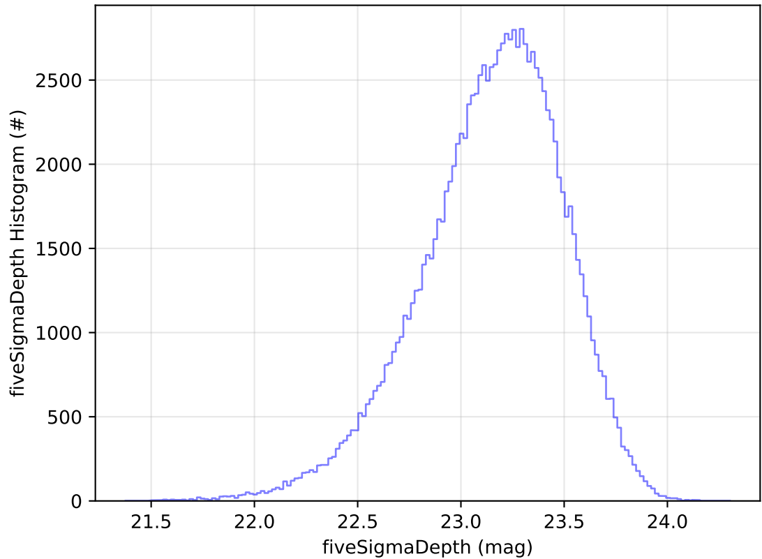
ddf_acor_sf10_lsf20_lsr10_v3.4_10yrs All sky u band: fiveSigmaDepth Histogram
