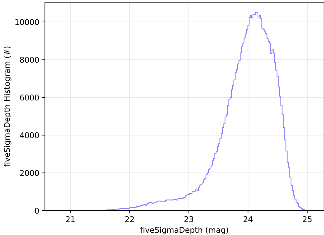
ddf_acor_sf10_lsf20_lsr10_v3.4_10yrs All sky r band: fiveSigmaDepth Histogram
