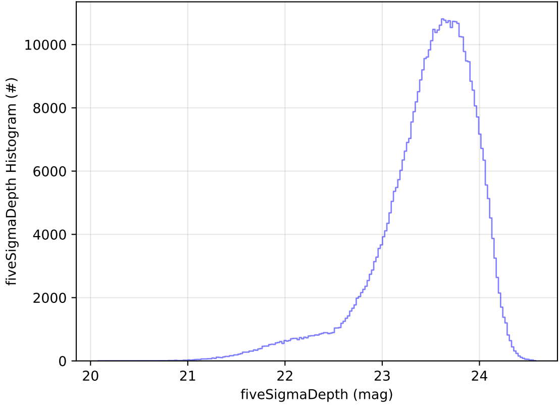
ddf_acor_sf10_lsf20_lsr10_v3.4_10yrs All sky i band: fiveSigmaDepth Histogram
