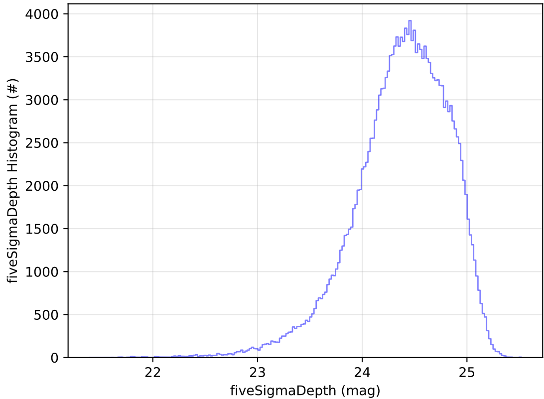
ddf_acor_sf10_lsf20_lsr10_v3.4_10yrs All sky g band: fiveSigmaDepth Histogram
