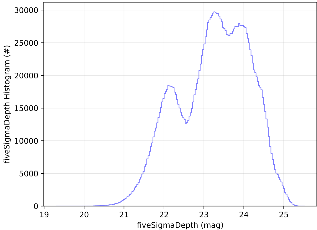
ddf_acor_sf10_lsf20_lsr10_v3.4_10yrs All sky all bands: fiveSigmaDepth Histogram
