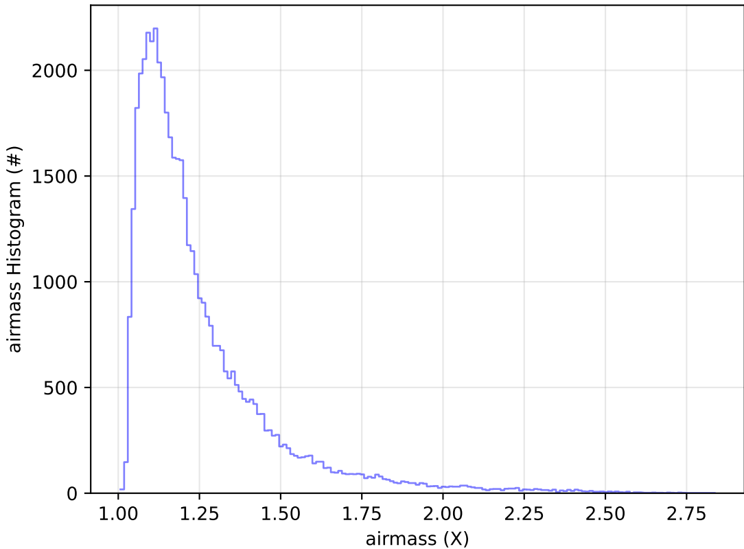
ddf_acor_sf10_ls20_lsr10_v3.4_10yrs Yr 1 y band: airmass Histogram
