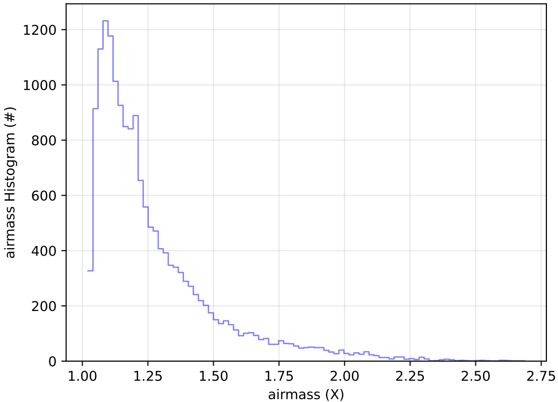
ddf_acor_sf10_lsf20_lsr10_v3.4_10yrs Yr 1 u band: airmass Histogram
