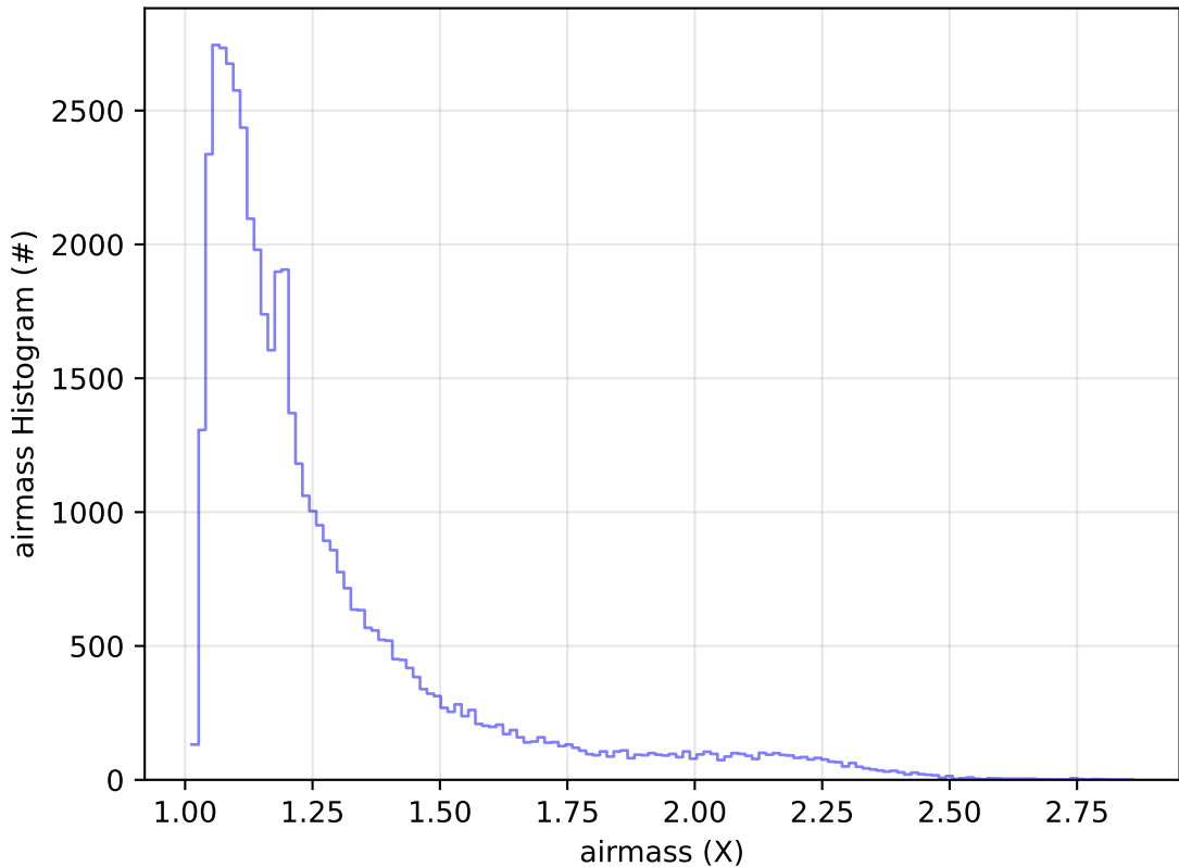
ddf_acor_sf10_lsf20_lsr10_v3.4_10yrs Yr 1 r band: airmass Histogram
