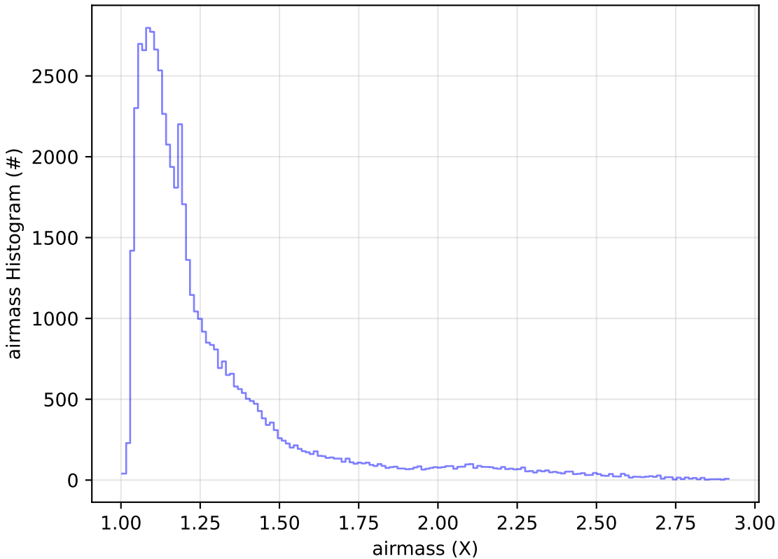
ddf_acor_sf10_lsf20_lsr10_v3.4_10yrs Yr 1 i band: airmass Histogram
