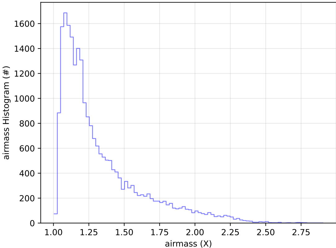
ddf_acor_sf10_lsf20_lsr10_v3.4_10yrs Yr 1 g band: airmass Histogram
