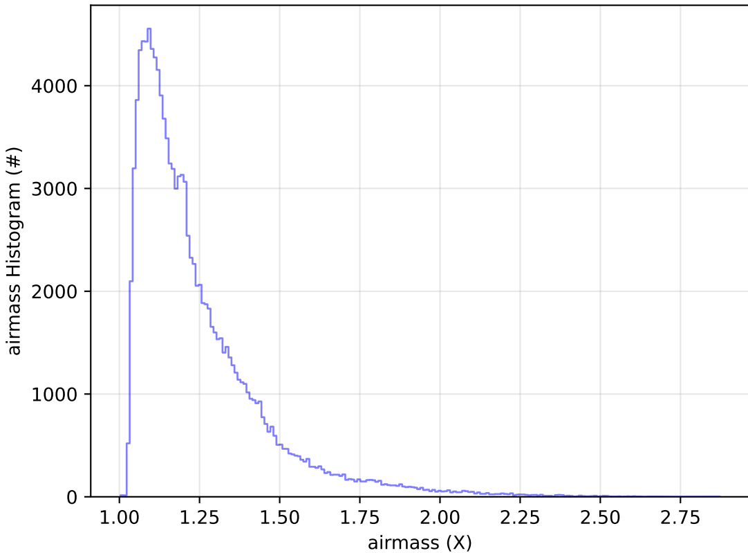
ddf_acor_sf10_lsf20_lsr10_v3.4_10yrs WFD u band: airmass Histogram
