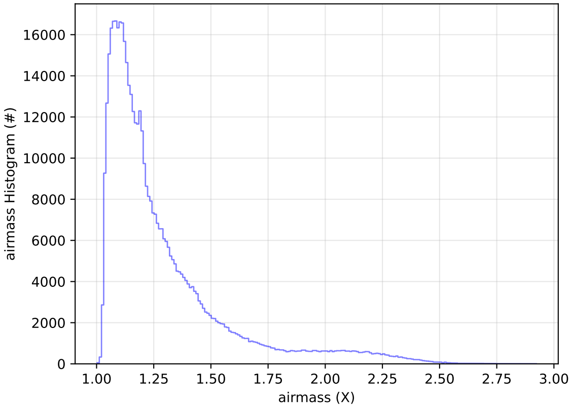
ddf_acor_sf10_lsf20_lsr10_v3.4_10yrs WFD r band: airmass Histogram
